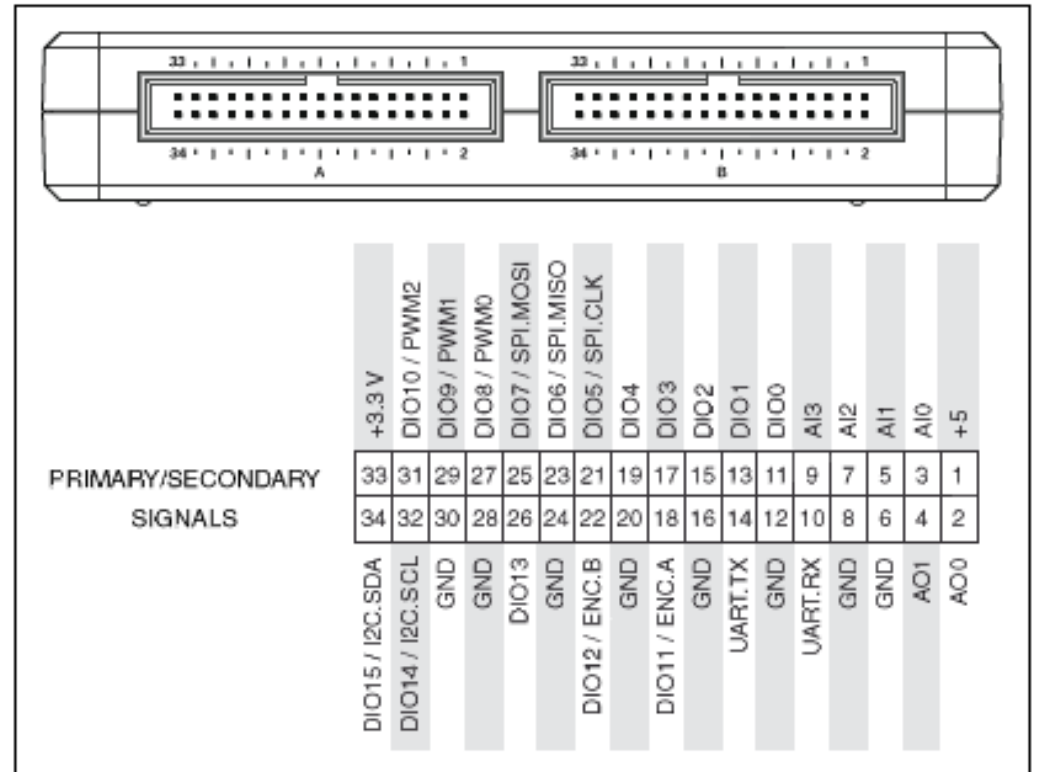
myRIO Extension Ports (MXP) Connectors
